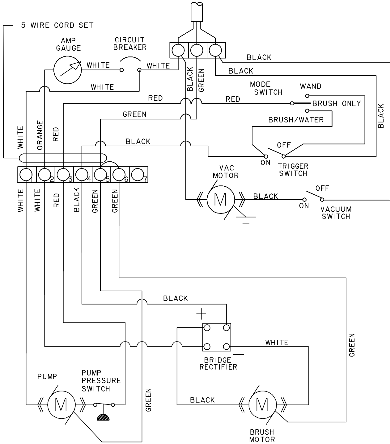
Fig. 6 – Electrical Schematic
